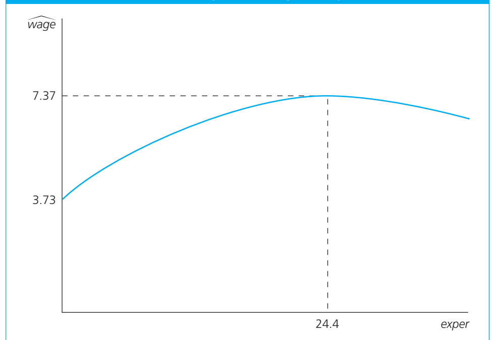
FIGURE 6.1 Quadratic relationship between \widehat{wage} and exper .
